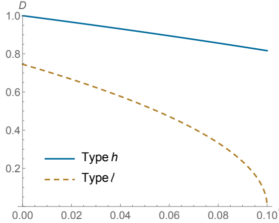
Figure 2: Optimal borrowing D_i as a function of the interest rate r for the two types h and l . The functional forms and parameter values used are the same as in Section 5 with \alpha(D) = 0.2D^2 and P = 0.8 .
